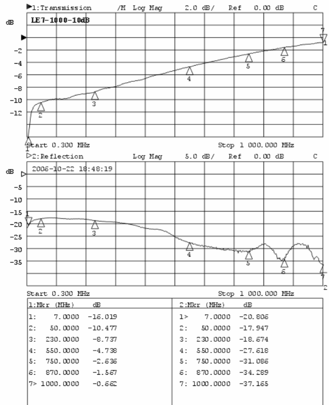
Model LE7-1000 -10dB Graph
